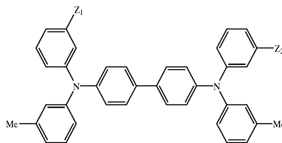
a triphenylamine derivative ("TPD") compound disclosed in J.Amer.Chem.Soc. 90 (1968) 3925
